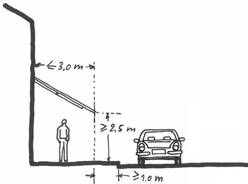
Figure 2 Saillies mobiles
